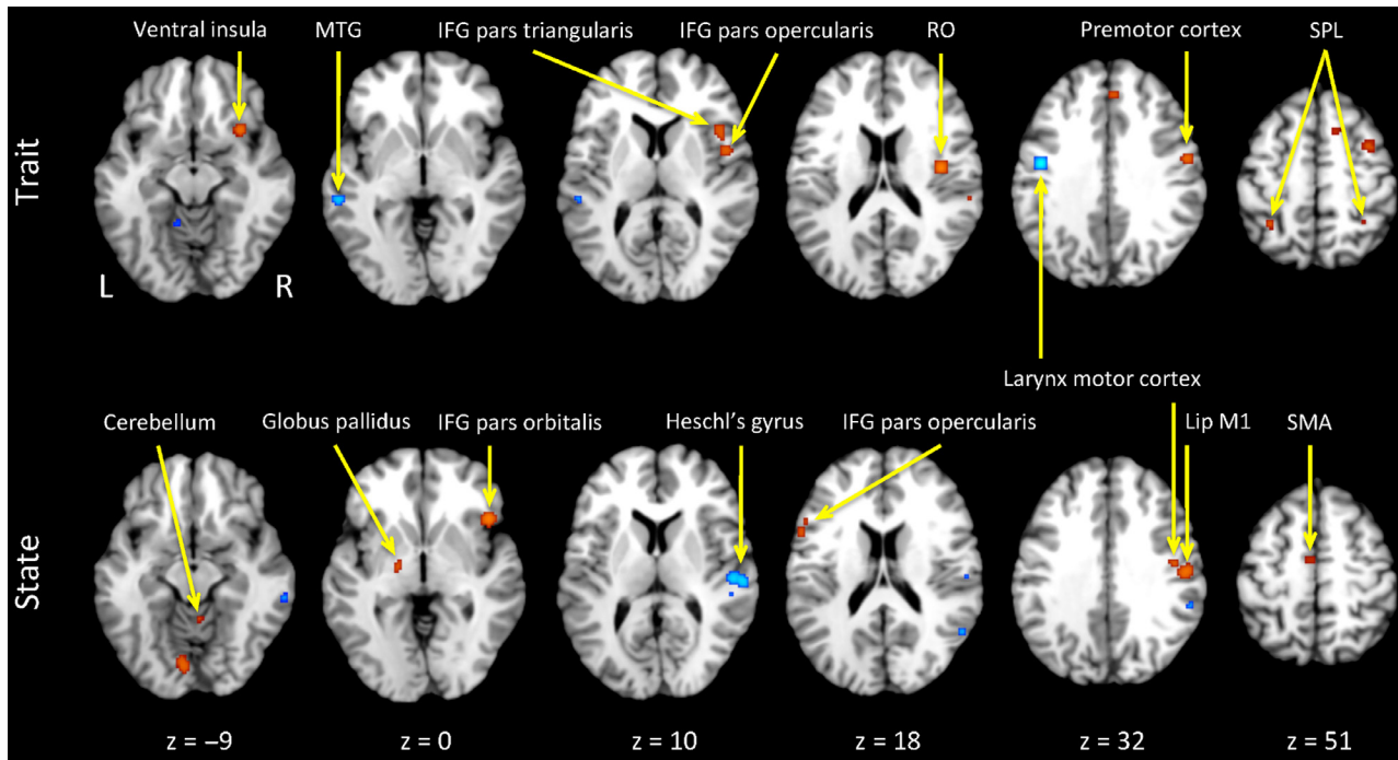
FIG. 2. Results of the ALE analyses. Axial slices in neurological convention showing regions consistently reported for trait and state stuttering. IFG, inferior frontal gyrus; MTG, middle temporal gyrus; RO, Rolandic operculum; SPL, superior parietal lobule; SMA, supplementary motor area.
