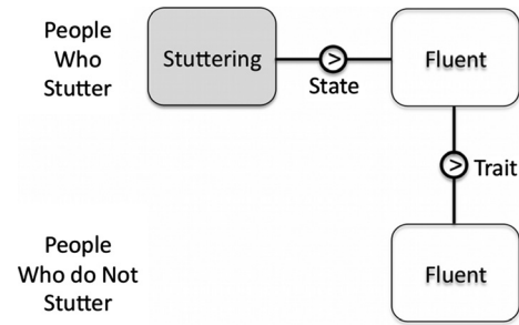
FIG. 1. Operational definitions of trait and state stuttering. Trait stuttering is revealed by contrasts between PWS and PWNS during fluent speech (PWS fluent > PWNS fluent). It is a between-group comparison. State stuttering is revealed by contrasts within PWS during stuttered vs. fluent speech (PWS stuttering > PWS fluent). It is a within-group comparison.
