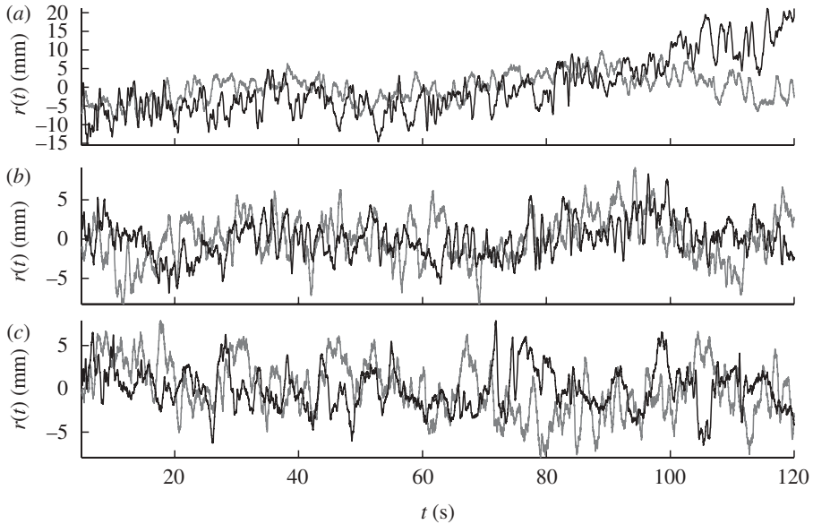
Figure 1. COP time series for (a) no vision, (b) 0 ms delay and (c) 750 ms delay. Grey line, data; black line, model.
