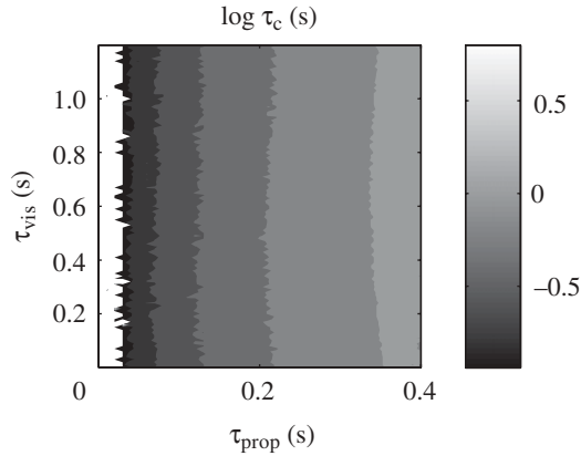
Figure 9. Critical time \tau_c as a function of proprioceptive delay \tau_{prop} and visual delay \tau_{vis} . White on this figure indicates that \tau_c does not exist between 0.1 and 10 s. The same parameters are used here as in figure 8, but with noise.
