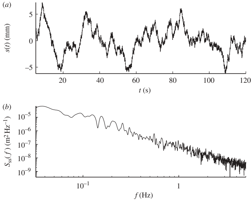
Figure 10. (a) A sample realization of s(t) for experimental visual delay of 750 ms and (b) its corresponding PSD.
