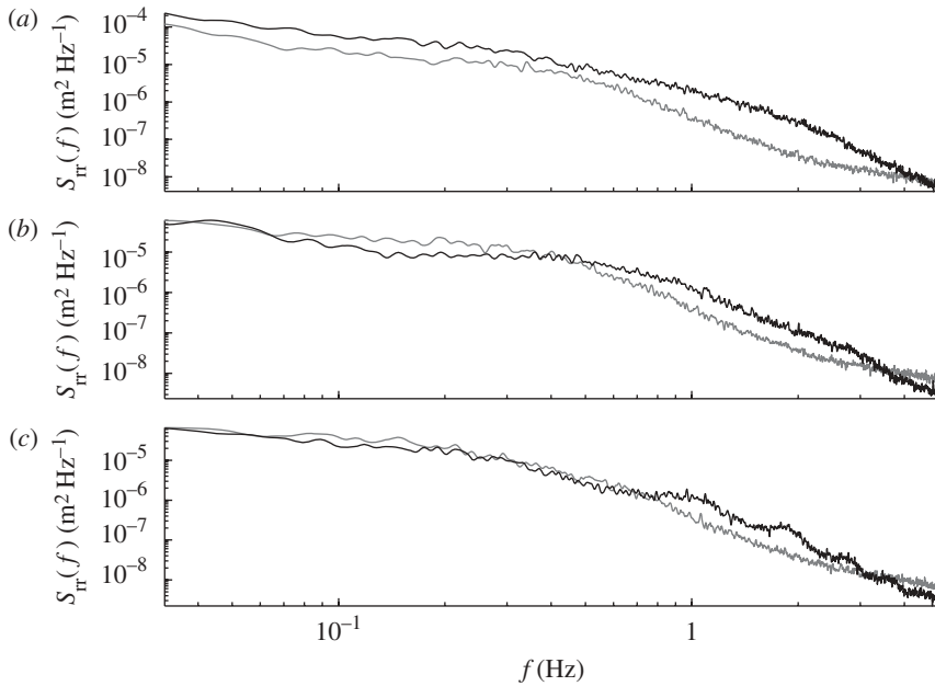
Figure 3. PSDs for (a) no vision, (b) 0 ms delay and (c) 750 ms delay. Grey line, data; black line, model.
