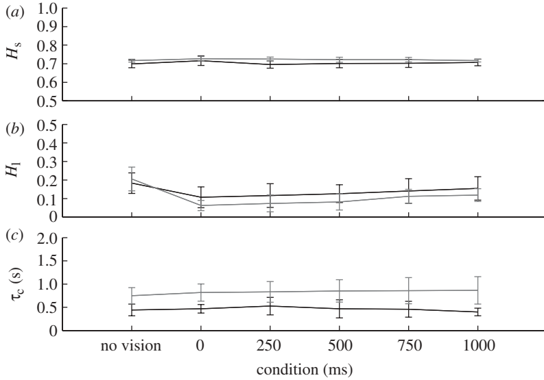
Figure 6. (a) Short- H_s and (b) long-range Hurst exponents H_l and (c) critical times. Black line, data; grey line, model.
