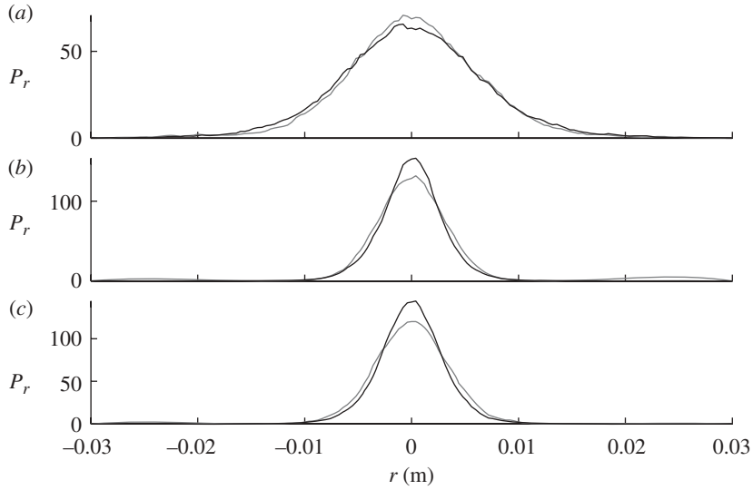
Figure 4. PDFs for (a) no vision, (b) 0 ms delay and (c) 750 ms delay. Grey line, data; black line, model.
