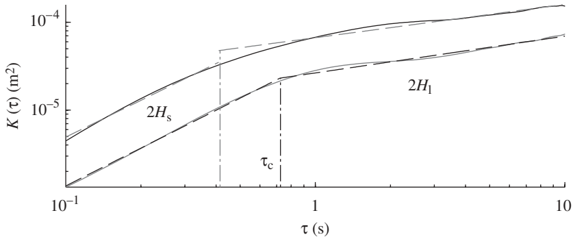
Figure 5. Mean-squared displacement for the no vision condition. Dotted line, data; bold line, model.
