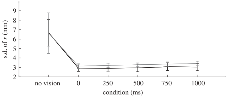
Figure 2. Standard deviation of COP times series for all conditions. Black line, data; grey line, model.
