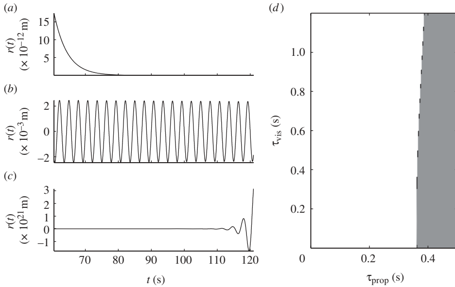
Figure 8. For all time series \tau_{\text{vis}} = 0.5 s and (a) \tau_{\text{prop}} = 0.2 s, (b) \tau_{\text{prop}} = 0.365 s and (c) \tau_{\text{prop}} = 0.450 s. (d) Stability diagrams: white, fixed point solution; black, marginally stable solution; grey, unbounded solution.
