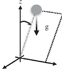
Figure 7. Inverted pendulum free-body diagram where x represents ML and y , AP.
